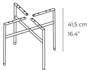
LEGS 260S (Black steel)
